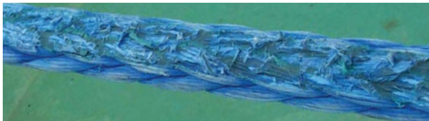
Melting damage on AmSteel®Blue.
